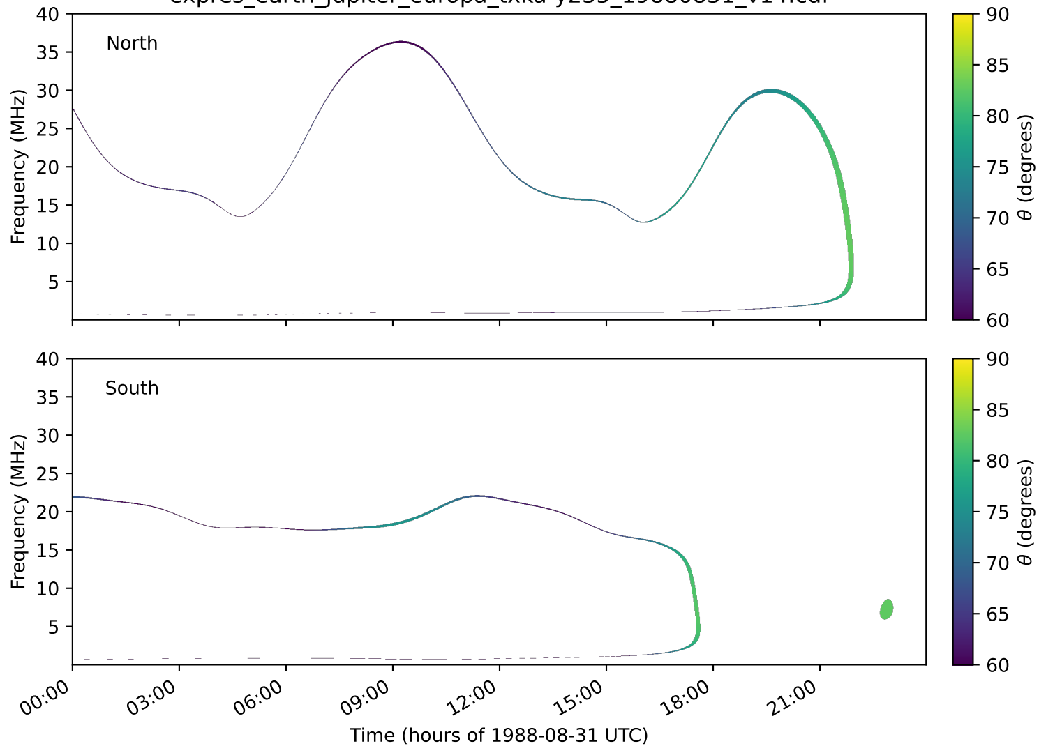
expres_earth_jupiter_europa_txka-y235_19880831_v14.cdf
