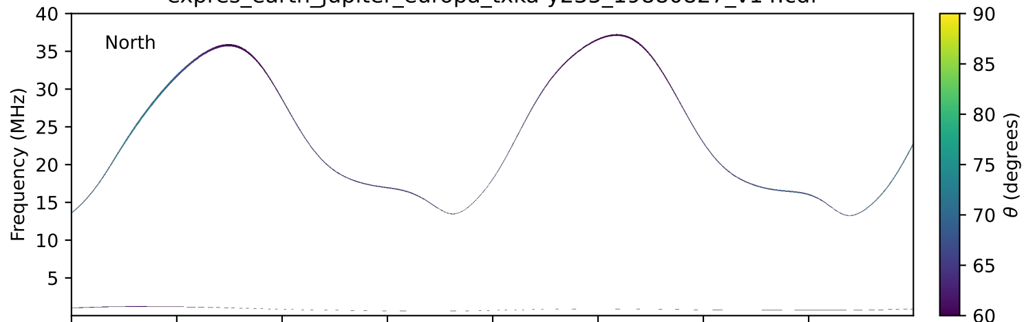
expres_earth_jupiter_europa_txka-y235_19880827_v14.cdf
