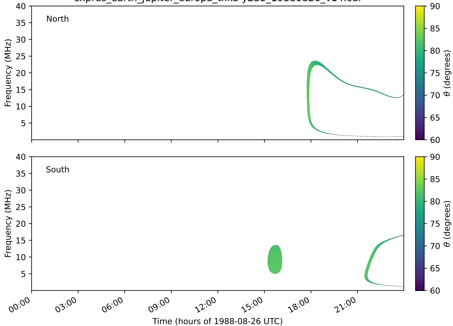
expres_earth_jupiter_europa_txka-y235_19880826_v14.cdf
