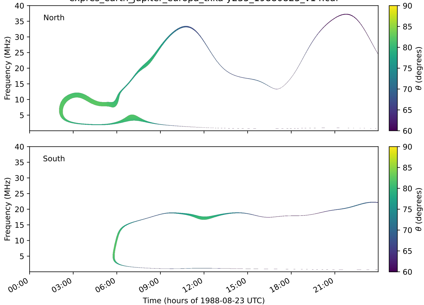
expres_earth_jupiter_europa_txka-y235_19880823_v14.cdf
