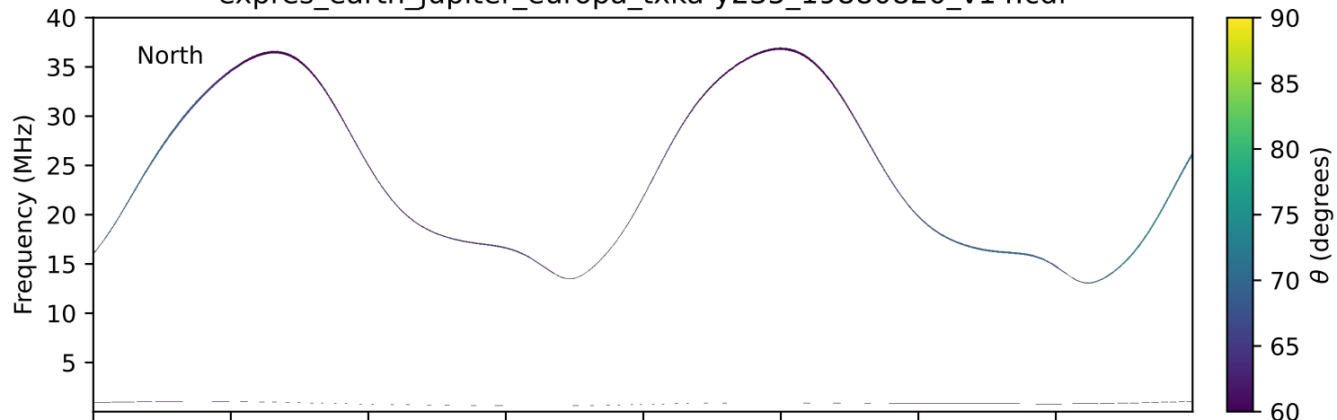
expres_earth_jupiter_europa_txka-y235_19880820_v14.cdf
