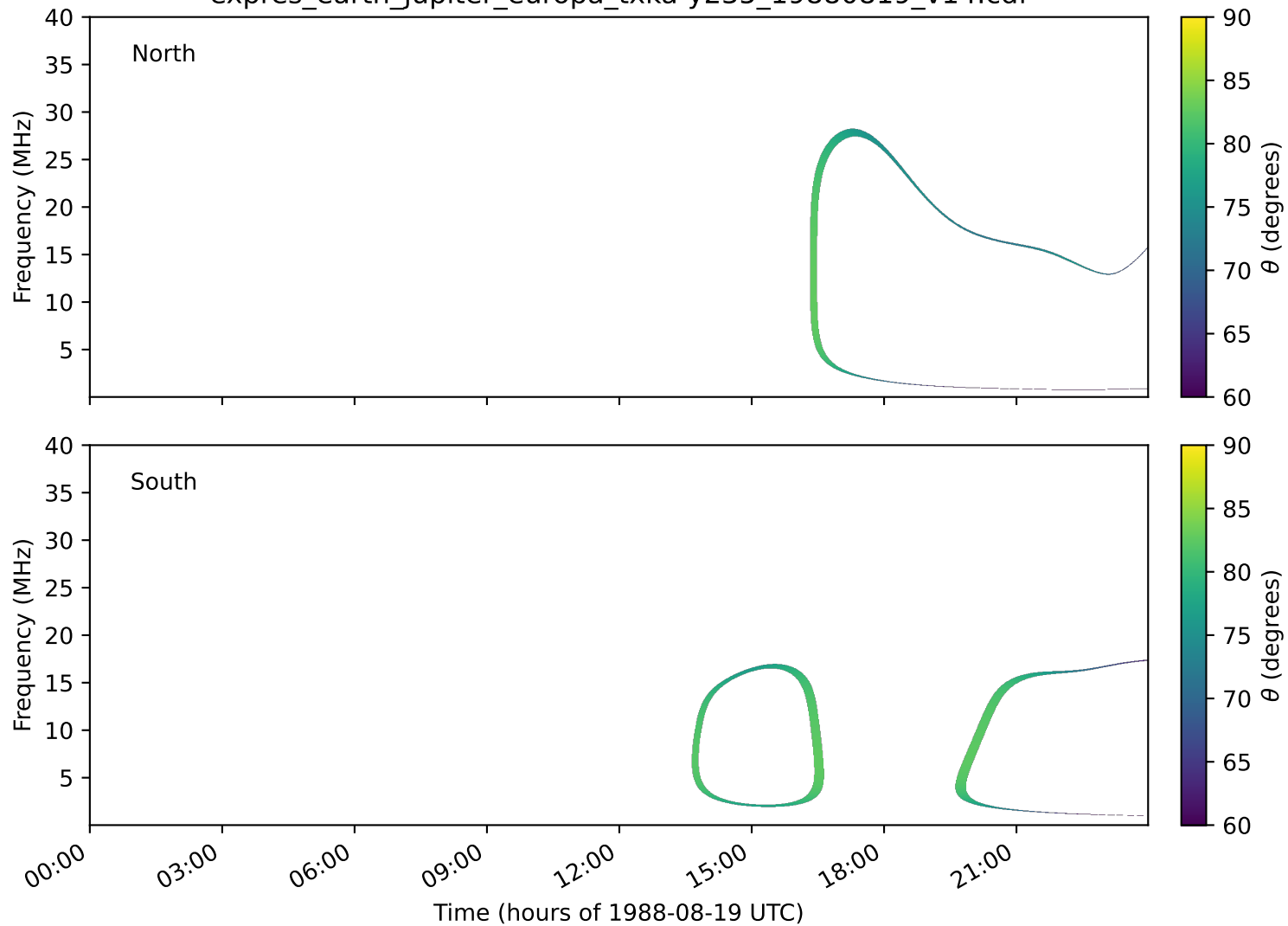
expres_earth_jupiter_europa_txka-y235_19880819_v14.cdf
