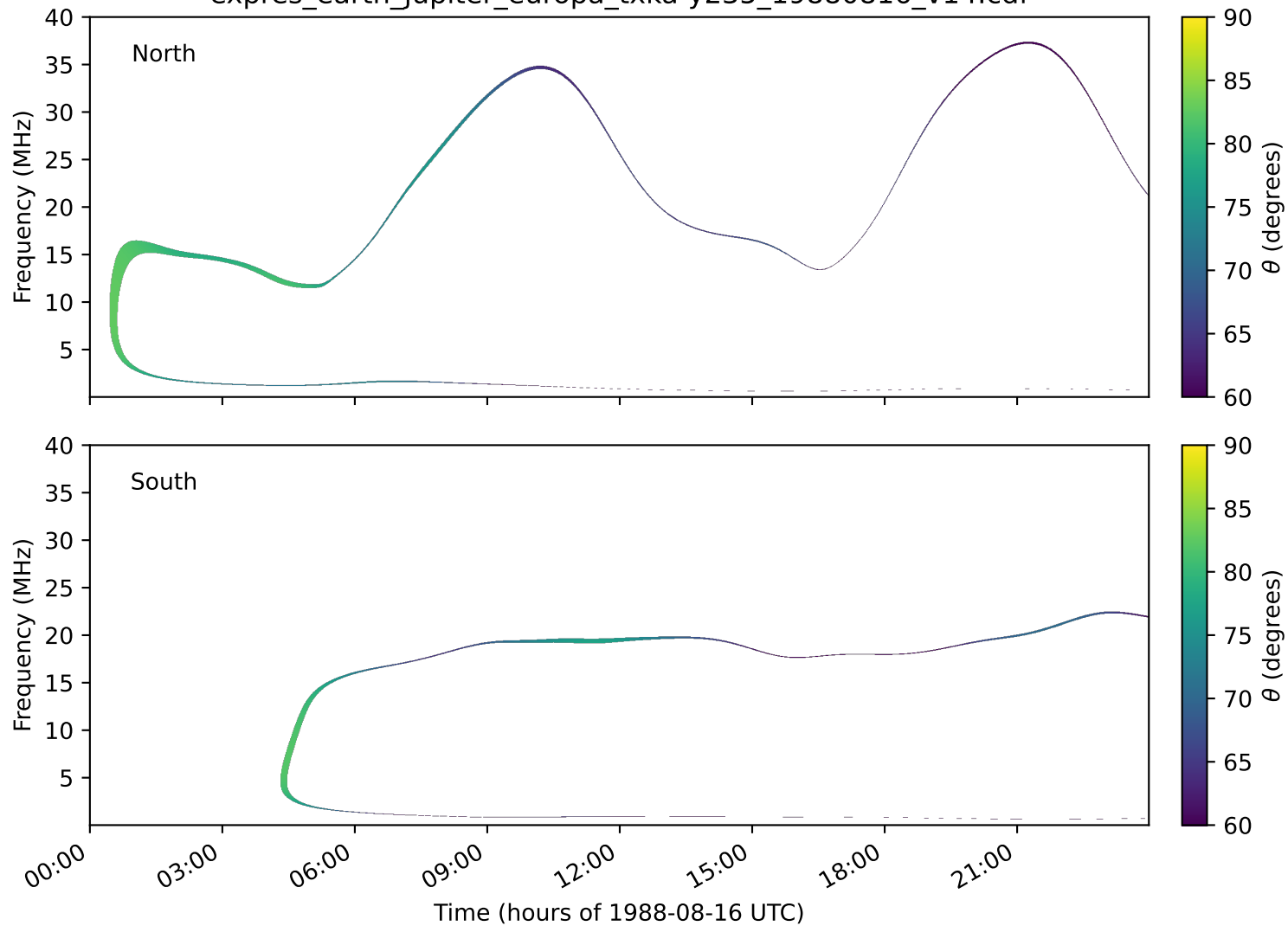
expres_earth_jupiter_europa_txka-y235_19880816_v14.cdf
