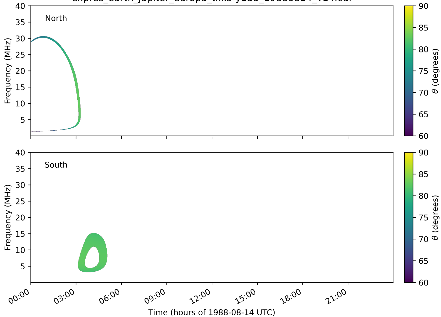
expres_earth_jupiter_europa_txka-y235_19880814_v14.cdf
