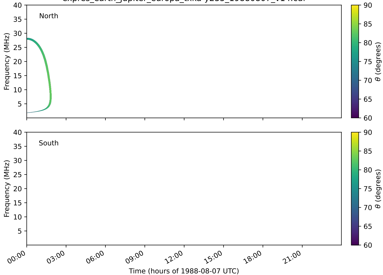
expres_earth_jupiter_europa_txka-y235_19880807_v14.cdf
