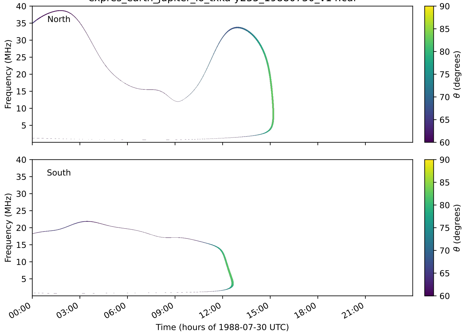
expres_earth_jupiter_io_txka-y235_19880730_v14.cdf
