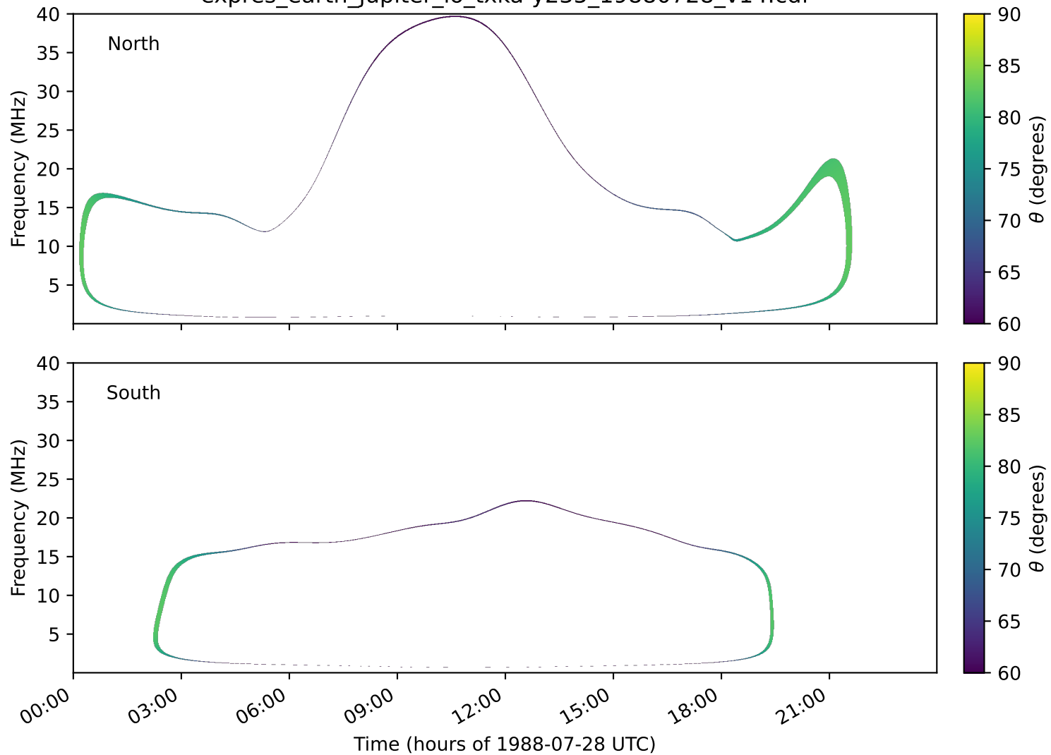
expres_earth_jupiter_io_txka-y235_19880728_v14.cdf
