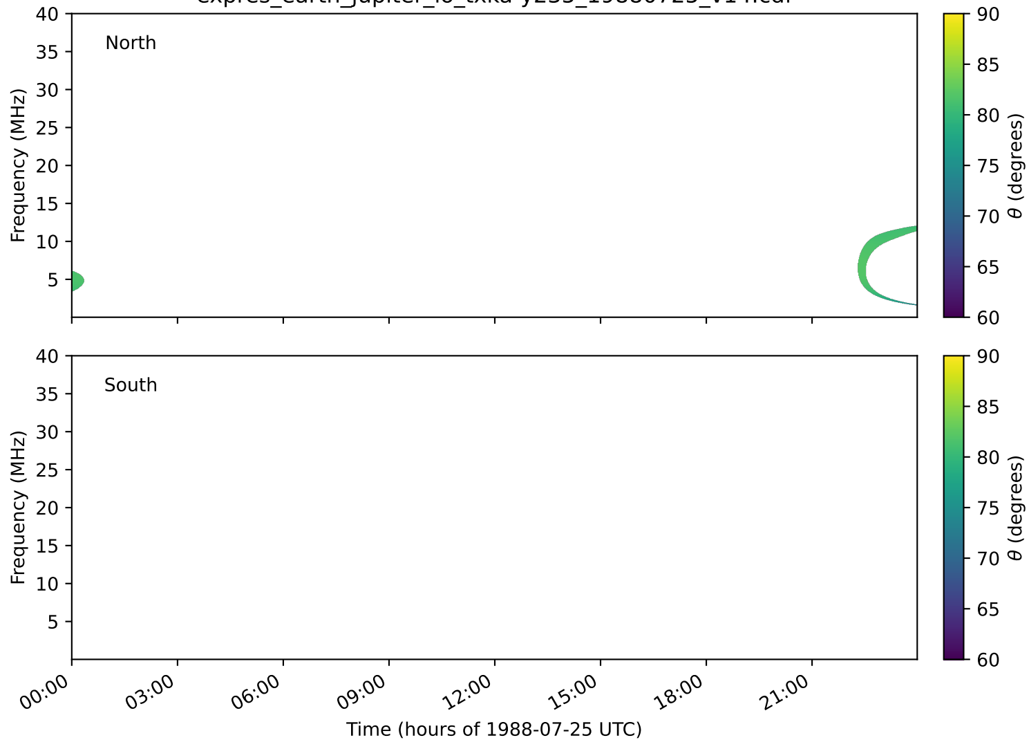
expres_earth_jupiter_io_txka-y235_19880725_v14.cdf
