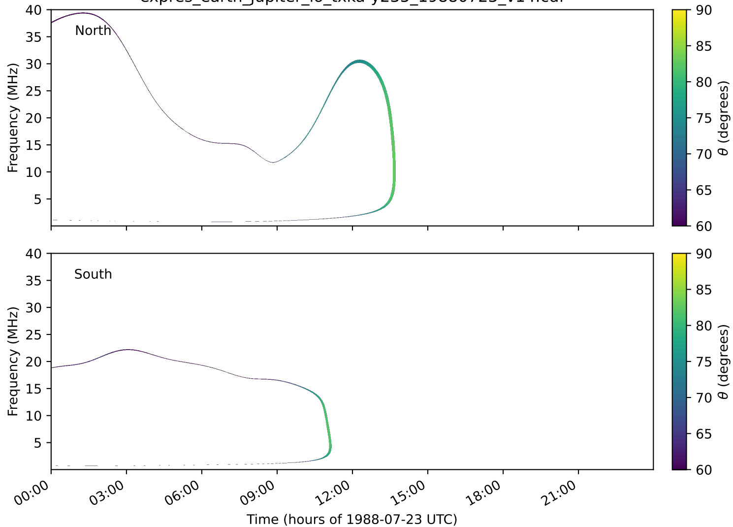
expres_earth_jupiter_io_txka-y235_19880723_v14.cdf
