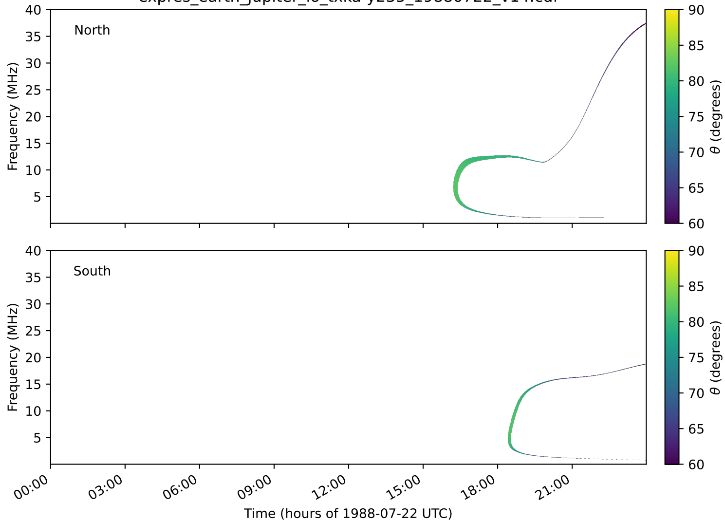
expres_earth_jupiter_io_txka-y235_19880722_v14.cdf
