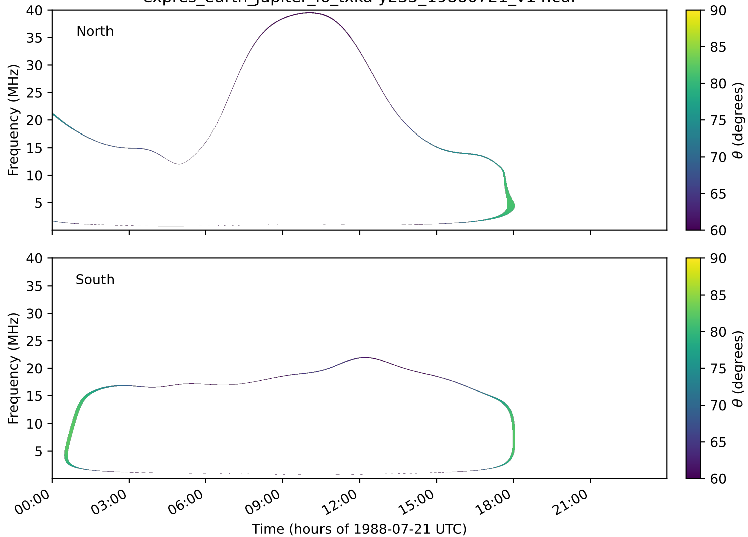
expres_earth_jupiter_io_txka-y235_19880721_v14.cdf
