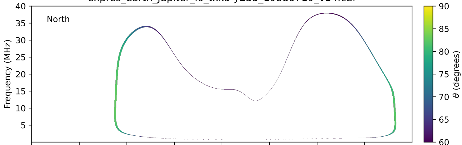
expres_earth_jupiter_io_txka-y235_19880719_v14.cdf
