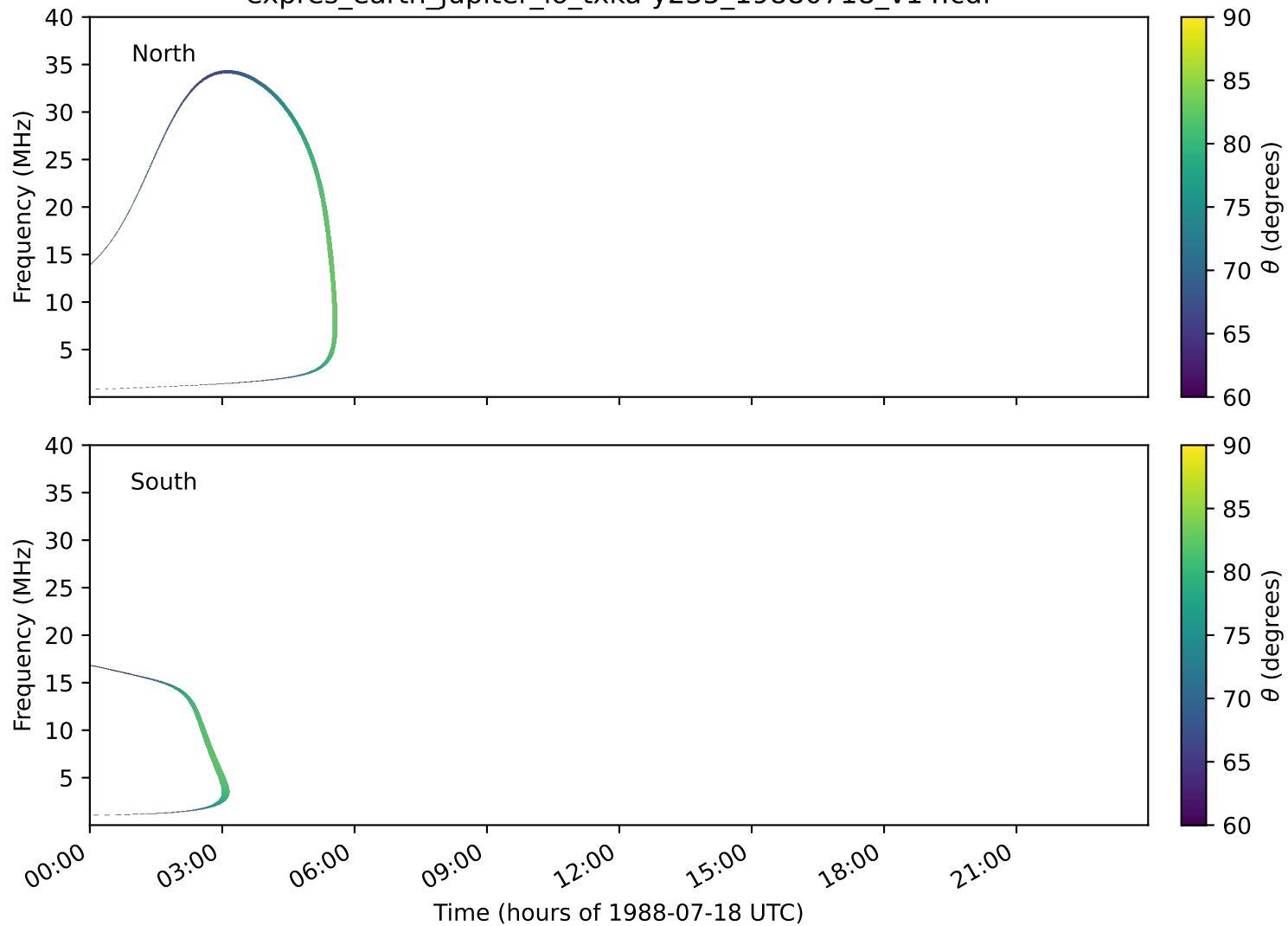
expres_earth_jupiter_io_txka-y235_19880718_v14.cdf
