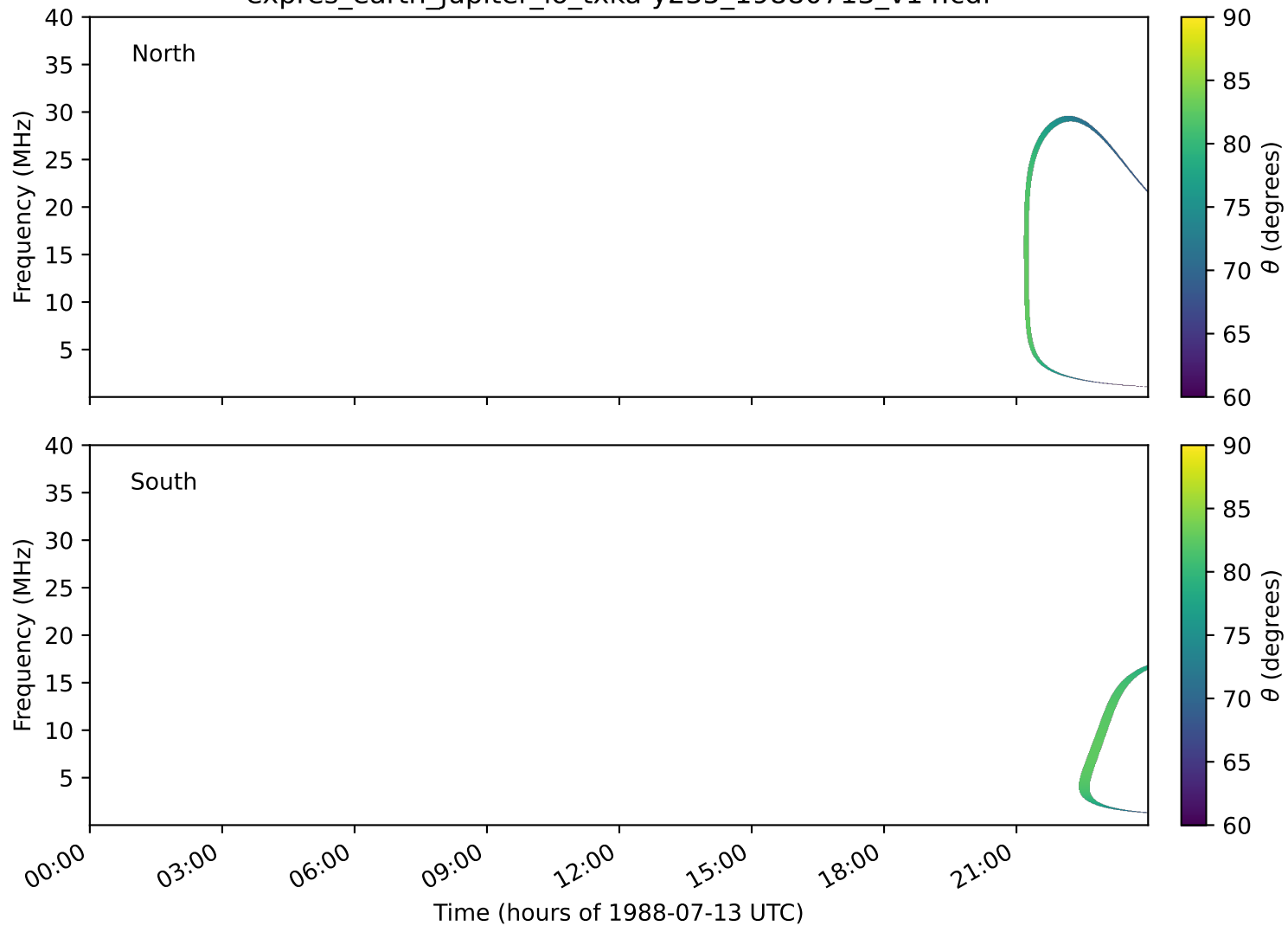
expres_earth_jupiter_io_txka-y235_19880713_v14.cdf
