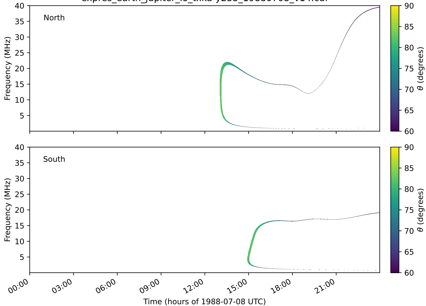
expres_earth_jupiter_io_txka-y235_19880708_v14.cdf
