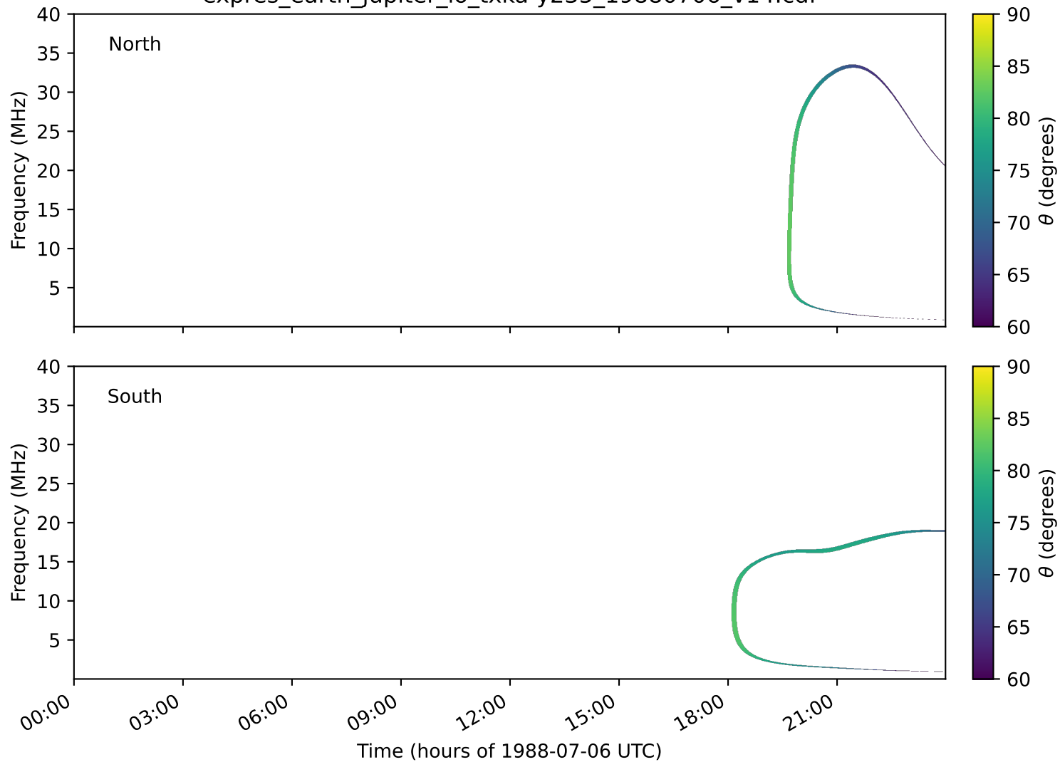
expres_earth_jupiter_io_txka-y235_19880706_v14.cdf
