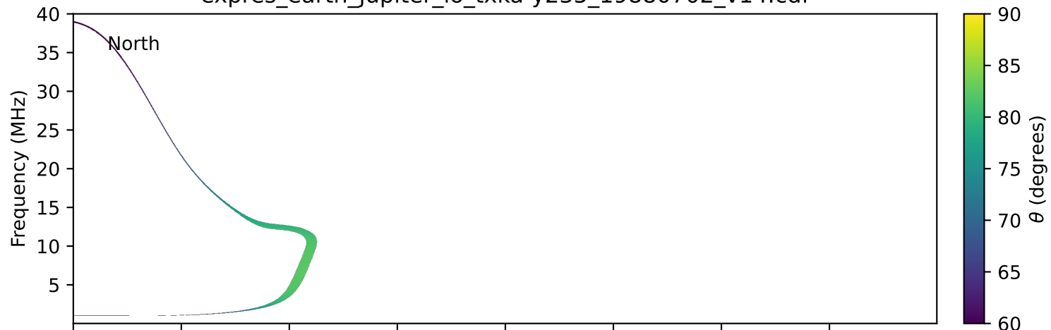
expres_earth_jupiter_io_txka-y235_19880702_v14.cdf
