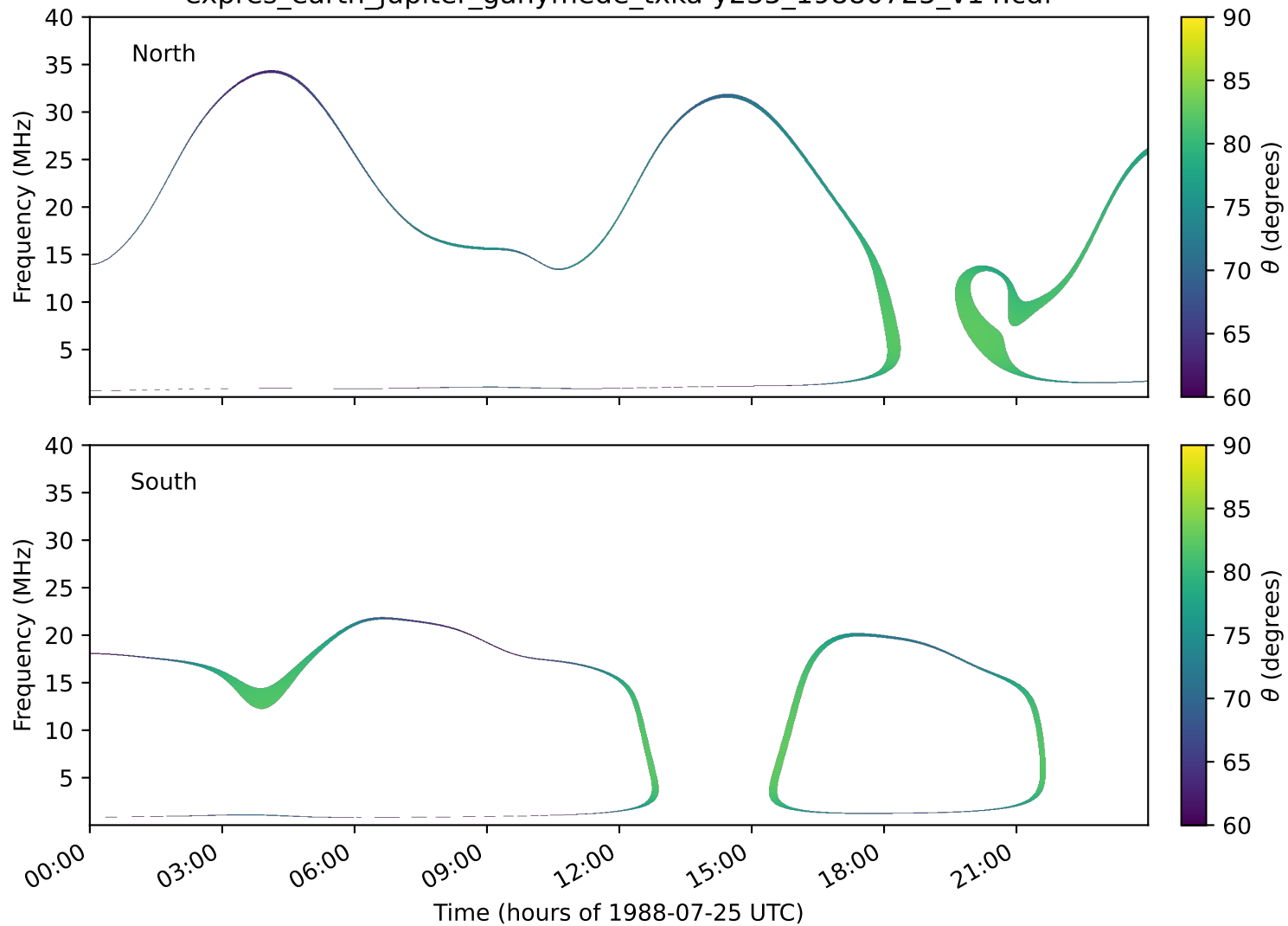
expres_earth_jupiter_ganymede_txka-y235_19880725_v14.cdf
