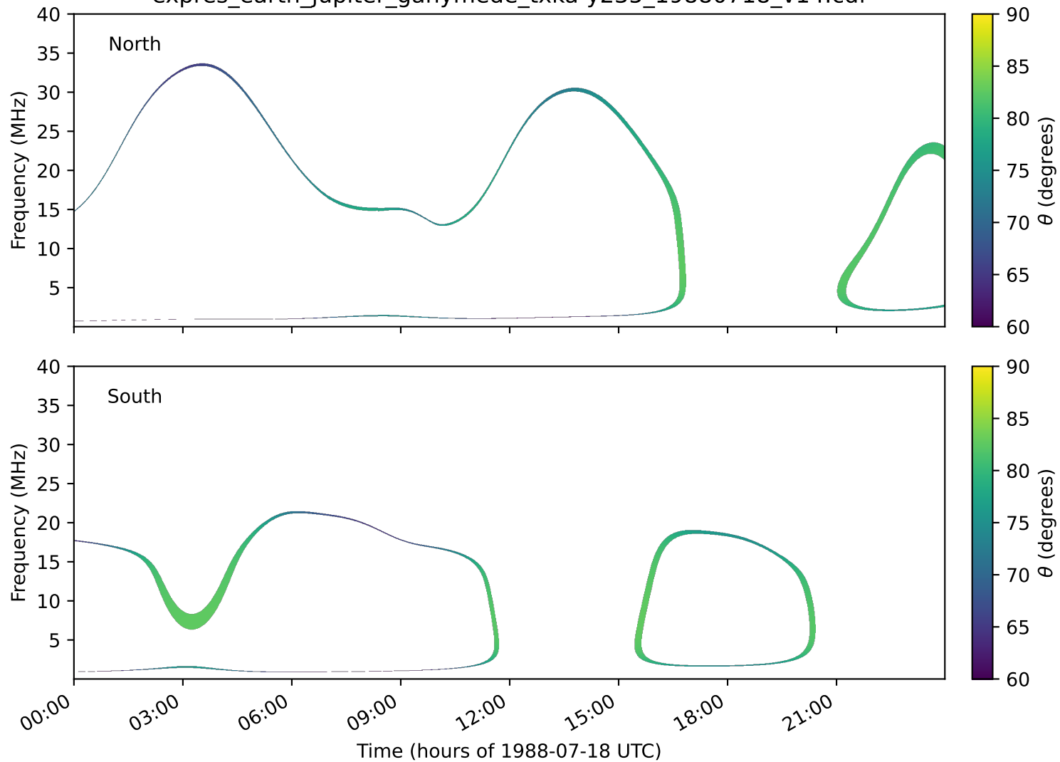
expres_earth_jupiter_ganymede_txka-y235_19880718_v14.cdf
