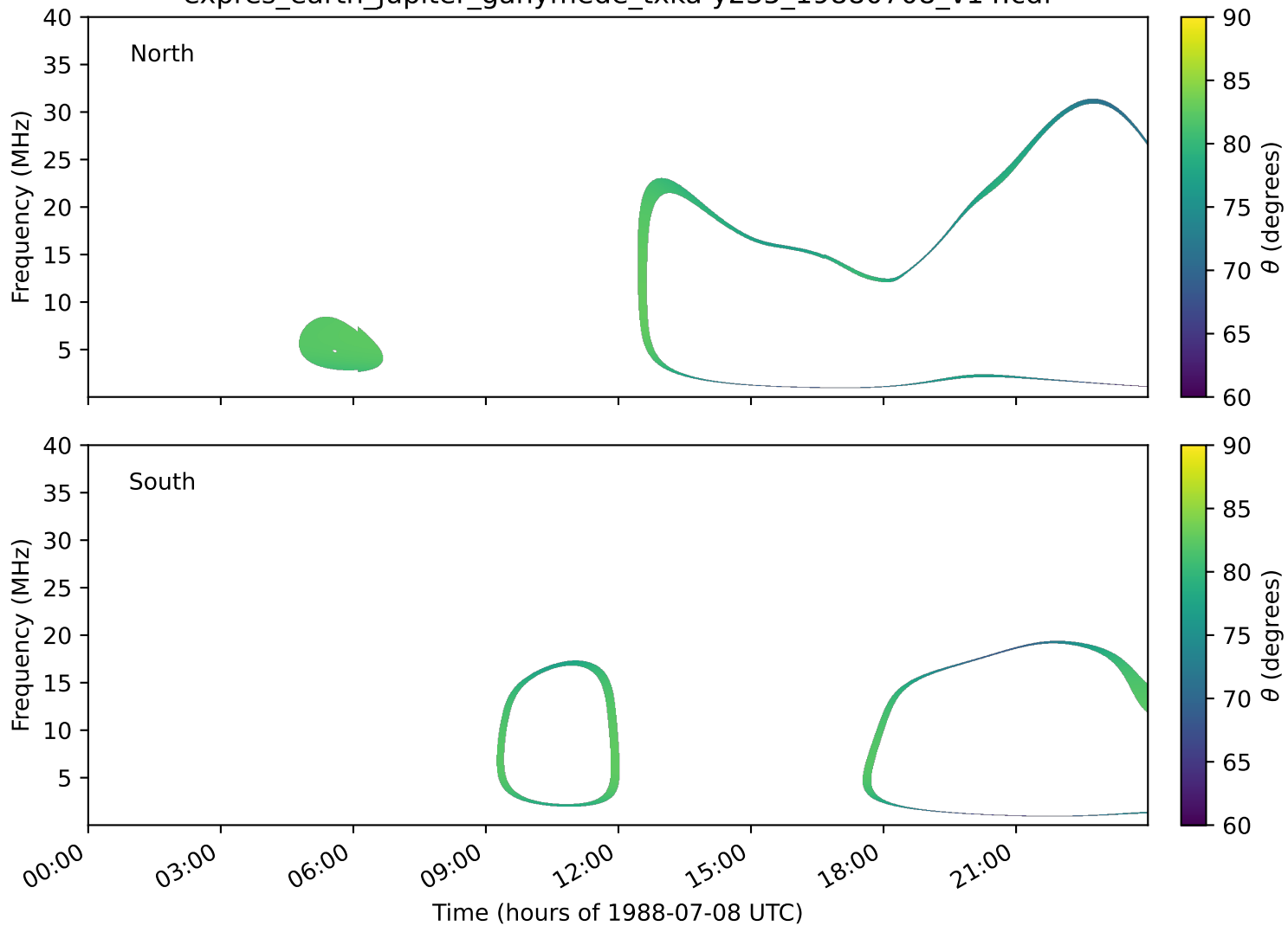
expres_earth_jupiter_ganymede_txka-y235_19880708_v14.cdf
