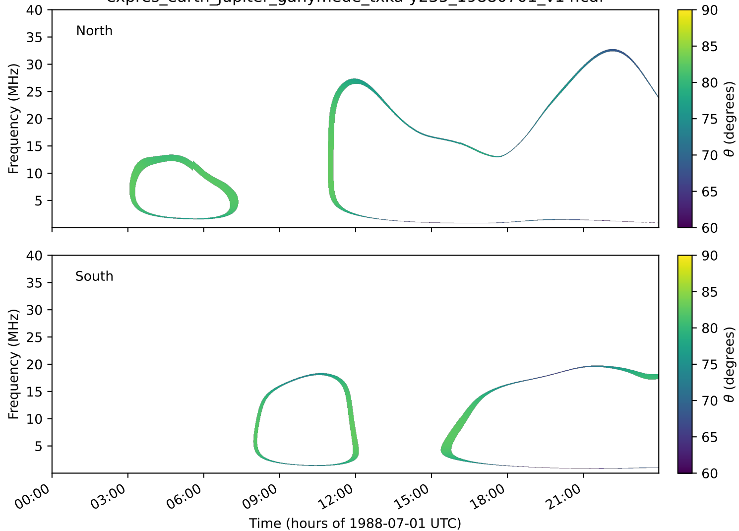
expres_earth_jupiter_ganymede_txka-y235_19880701_v14.cdf
