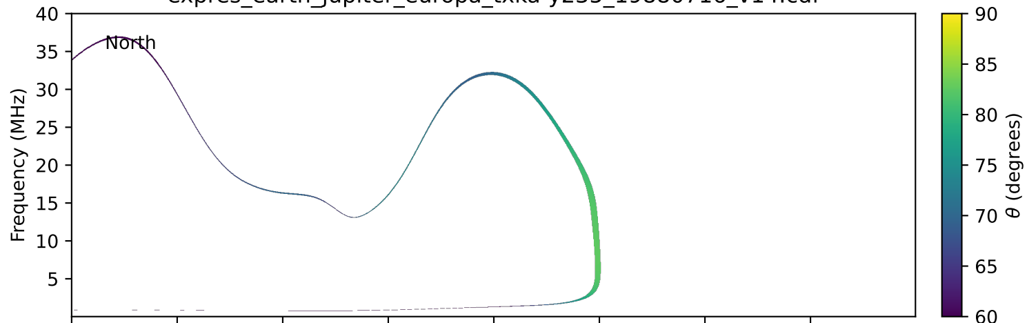
expres_earth_jupiter_europa_txka-y235_19880716_v14.cdf
