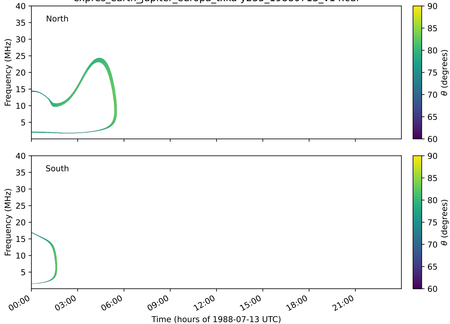
expres_earth_jupiter_europa_txka-y235_19880713_v14.cdf
