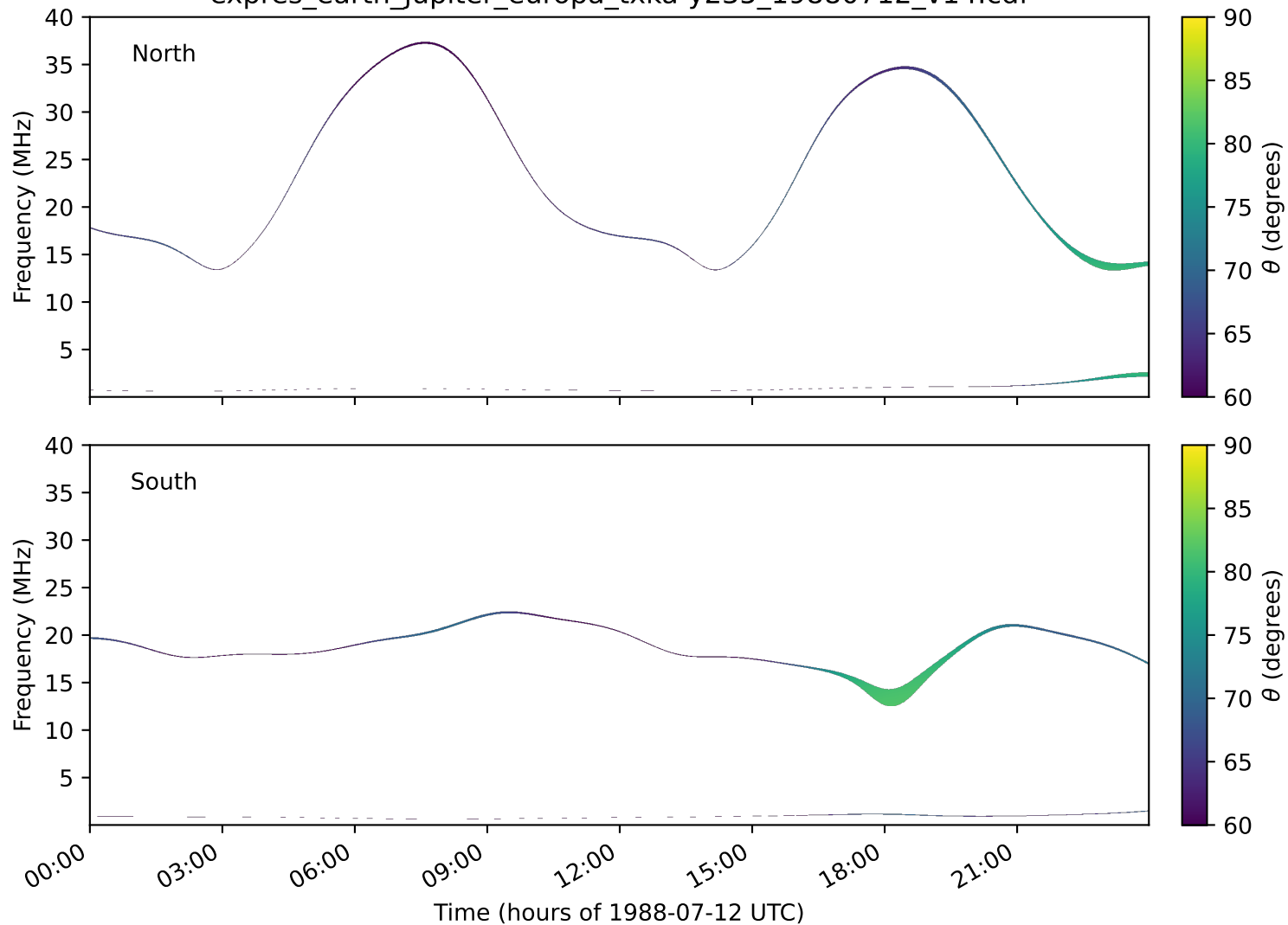
expres_earth_jupiter_europa_txka-y235_19880712_v14.cdf
