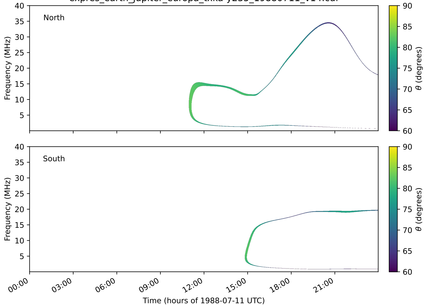
expres_earth_jupiter_europa_txka-y235_19880711_v14.cdf
