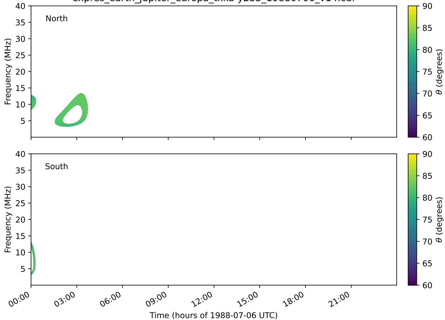
expres_earth_jupiter_europa_txka-y235_19880706_v14.cdf
