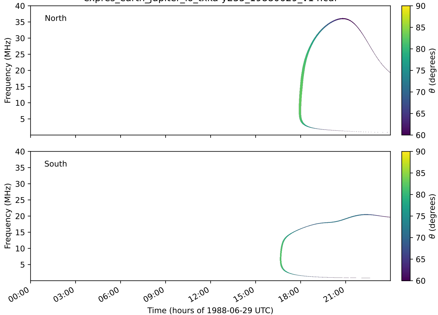
expres_earth_jupiter_io_txka-y235_19880629_v14.cdf
