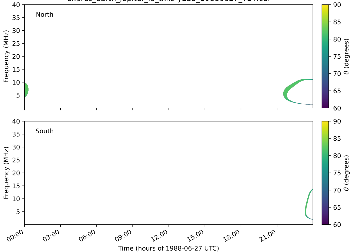
expres_earth_jupiter_io_txka-y235_19880627_v14.cdf
