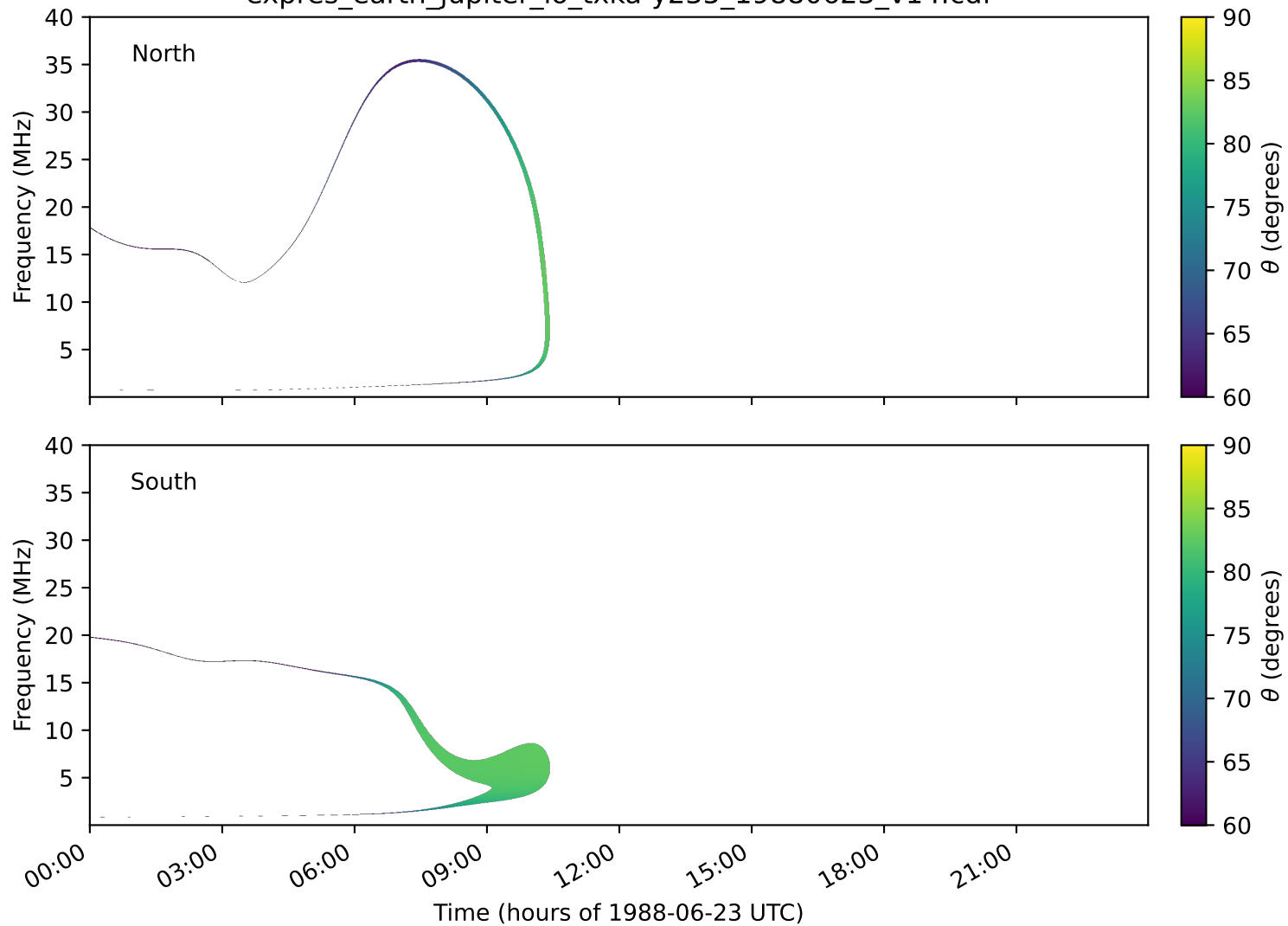
expres_earth_jupiter_io_txka-y235_19880623_v14.cdf
