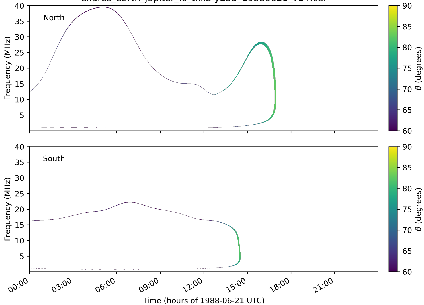
expres_earth_jupiter_io_txka-y235_19880621_v14.cdf
