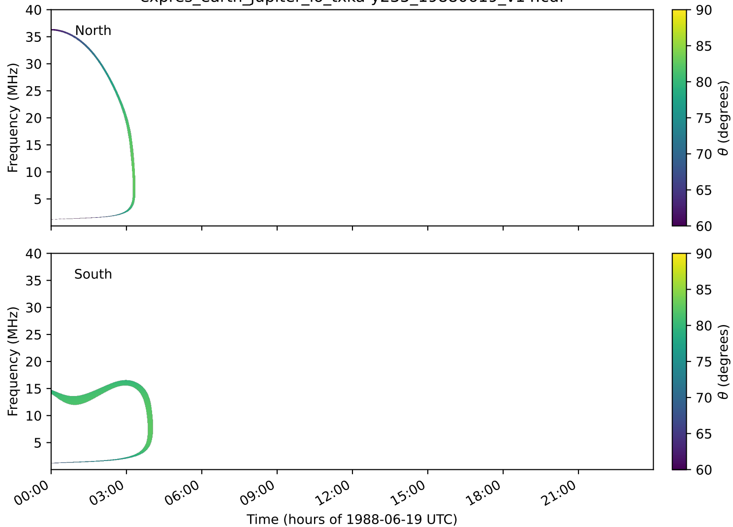
expres_earth_jupiter_io_txka-y235_19880619_v14.cdf
