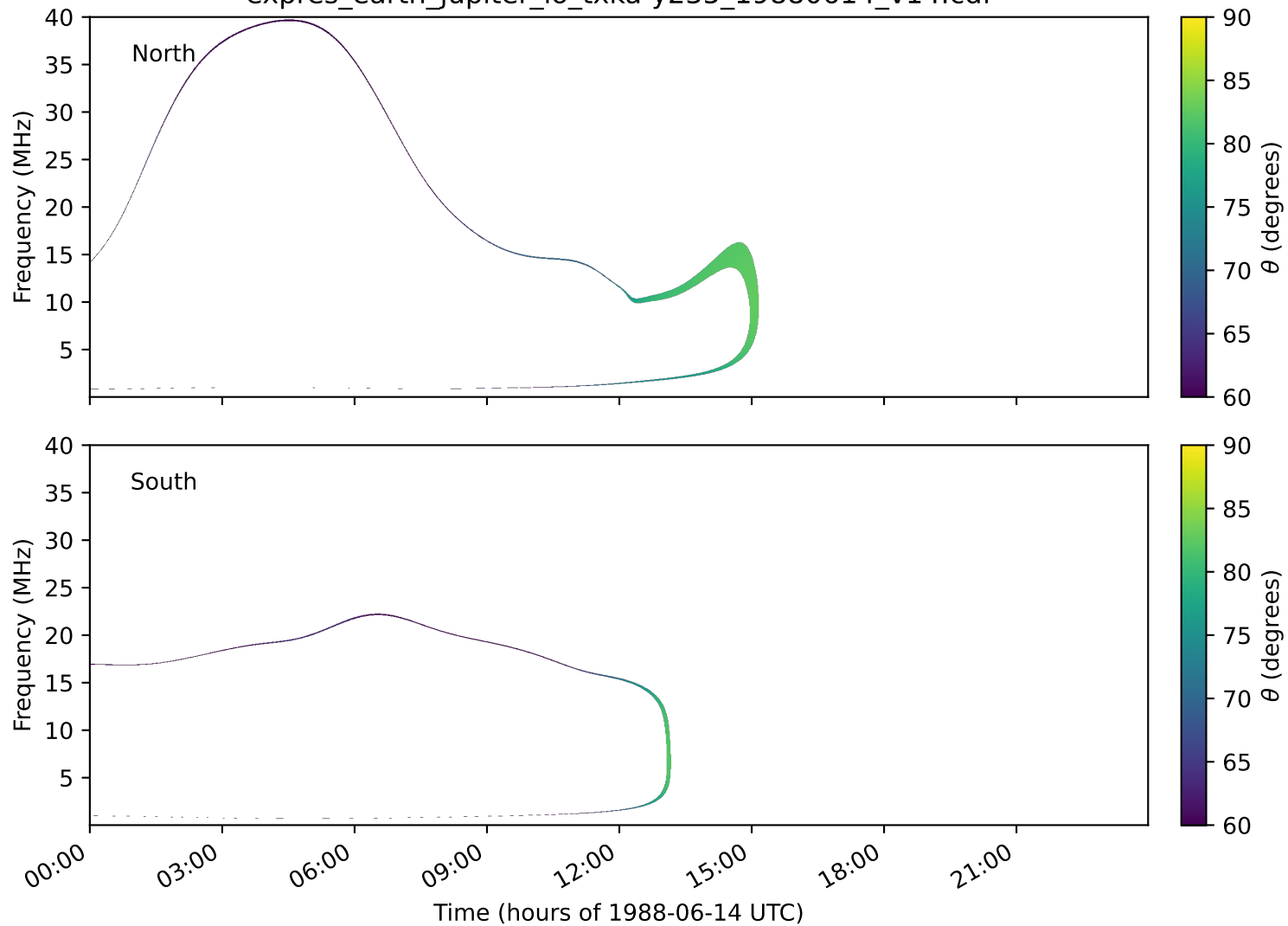
expres_earth_jupiter_io_txka-y235_19880614_v14.cdf
