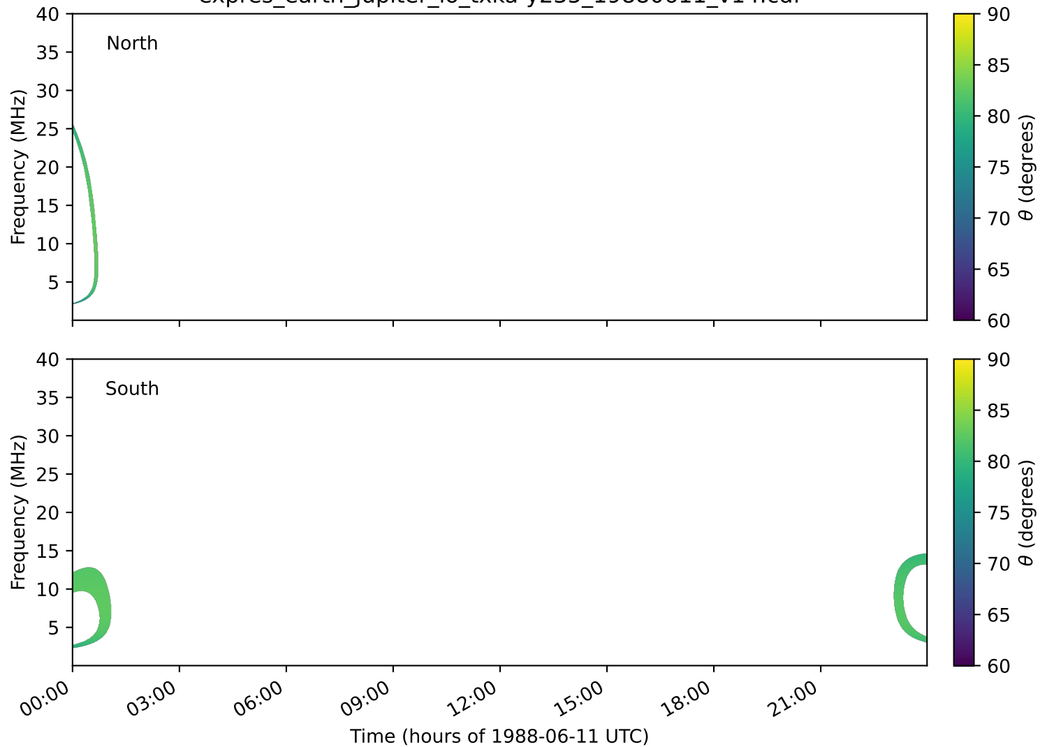
expres_earth_jupiter_io_txka-y235_19880611_v14.cdf
