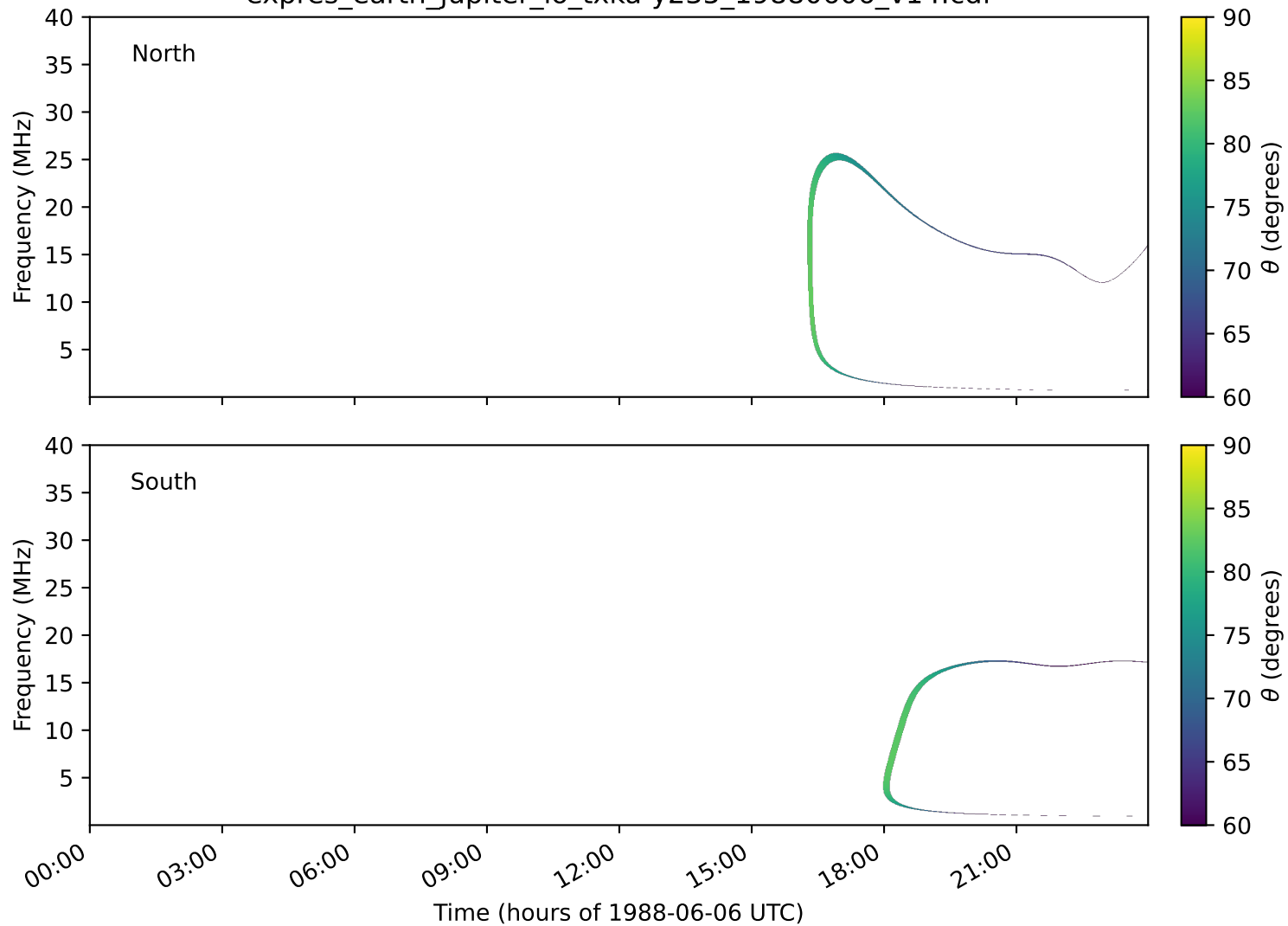
expres_earth_jupiter_io_txka-y235_19880606_v14.cdf
