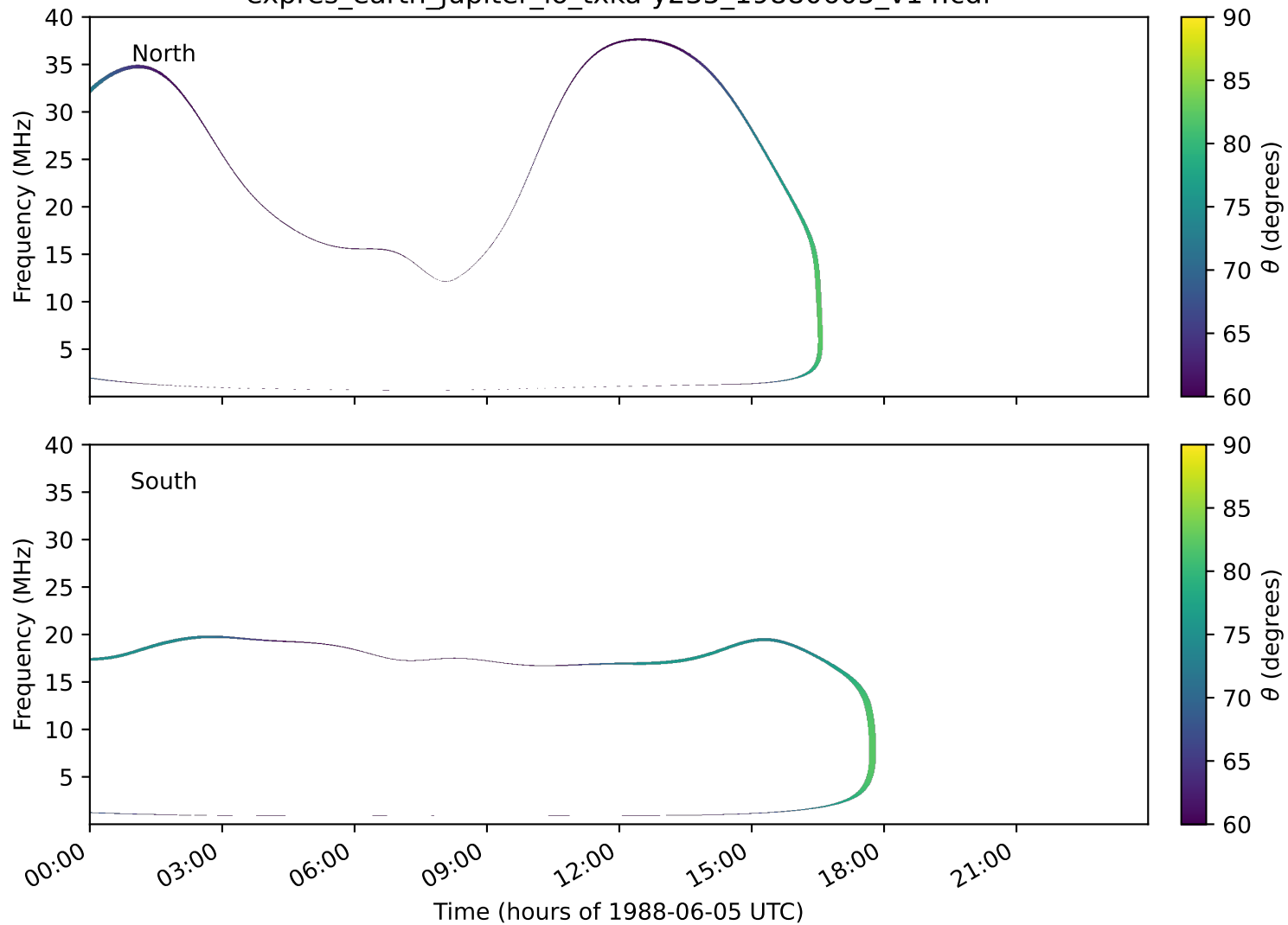
expres_earth_jupiter_io_txka-y235_19880605_v14.cdf
