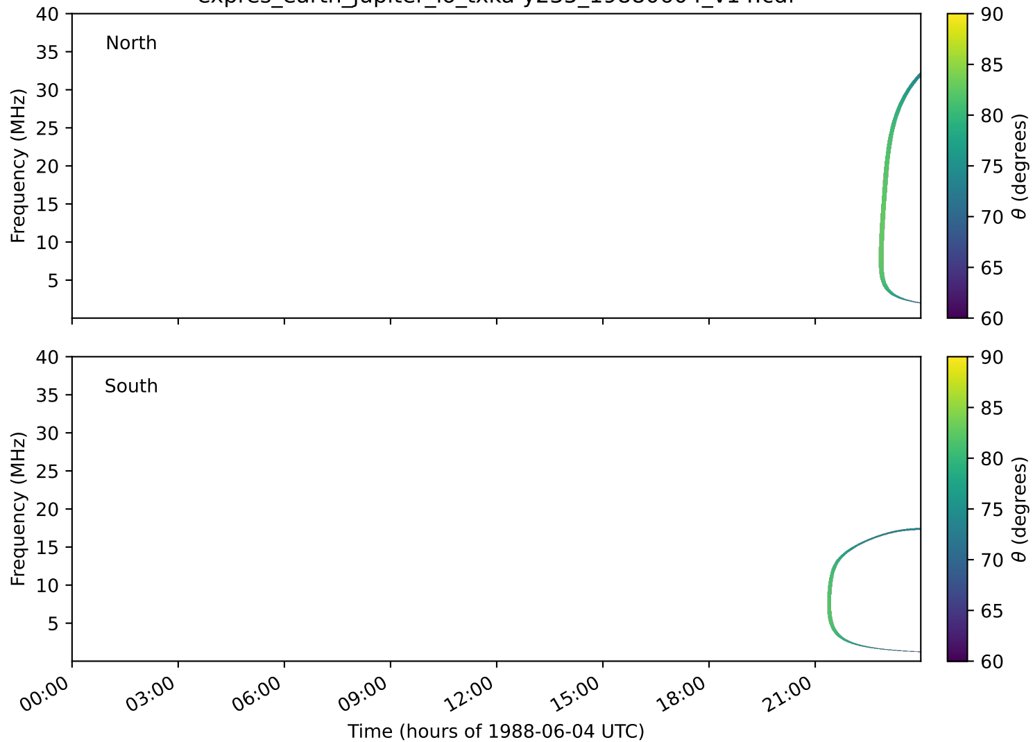
expres_earth_jupiter_io_txka-y235_19880604_v14.cdf
