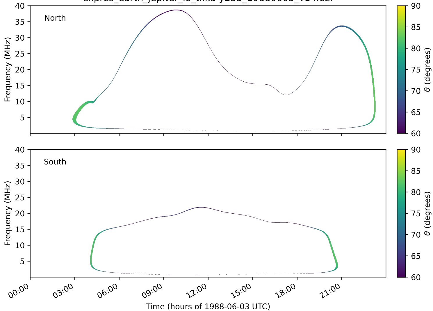
expres_earth_jupiter_io_txka-y235_19880603_v14.cdf
