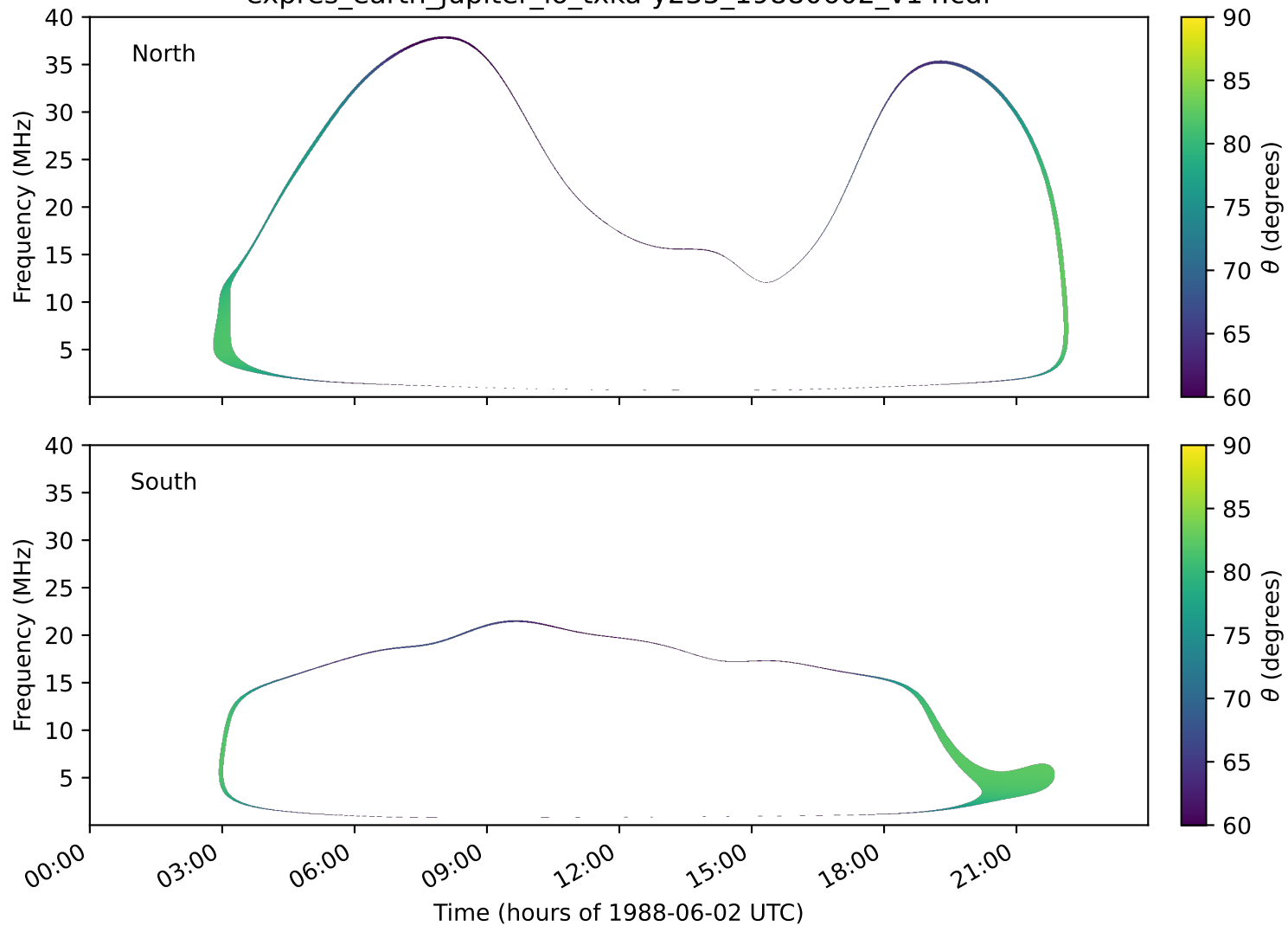
expres_earth_jupiter_io_txka-y235_19880602_v14.cdf
