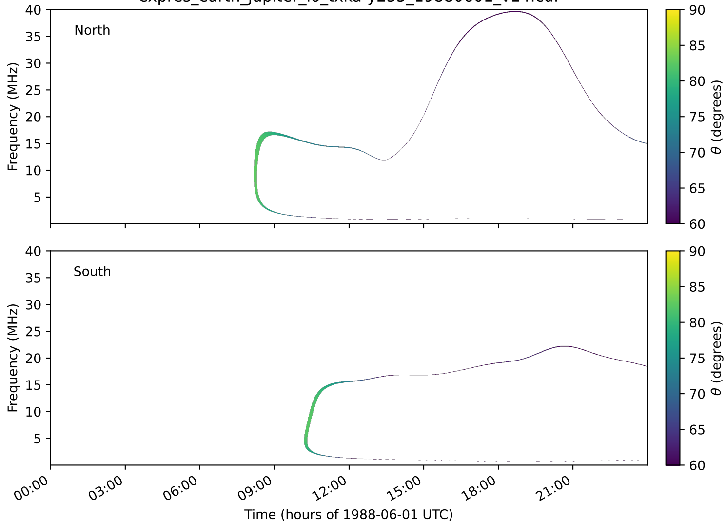
expres_earth_jupiter_io_txka-y235_19880601_v14.cdf
