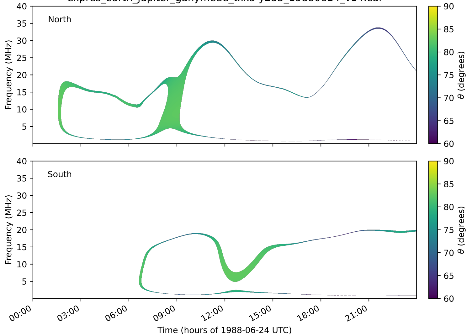
expres_earth_jupiter_ganymede_txka-y235_19880624_v14.cdf
