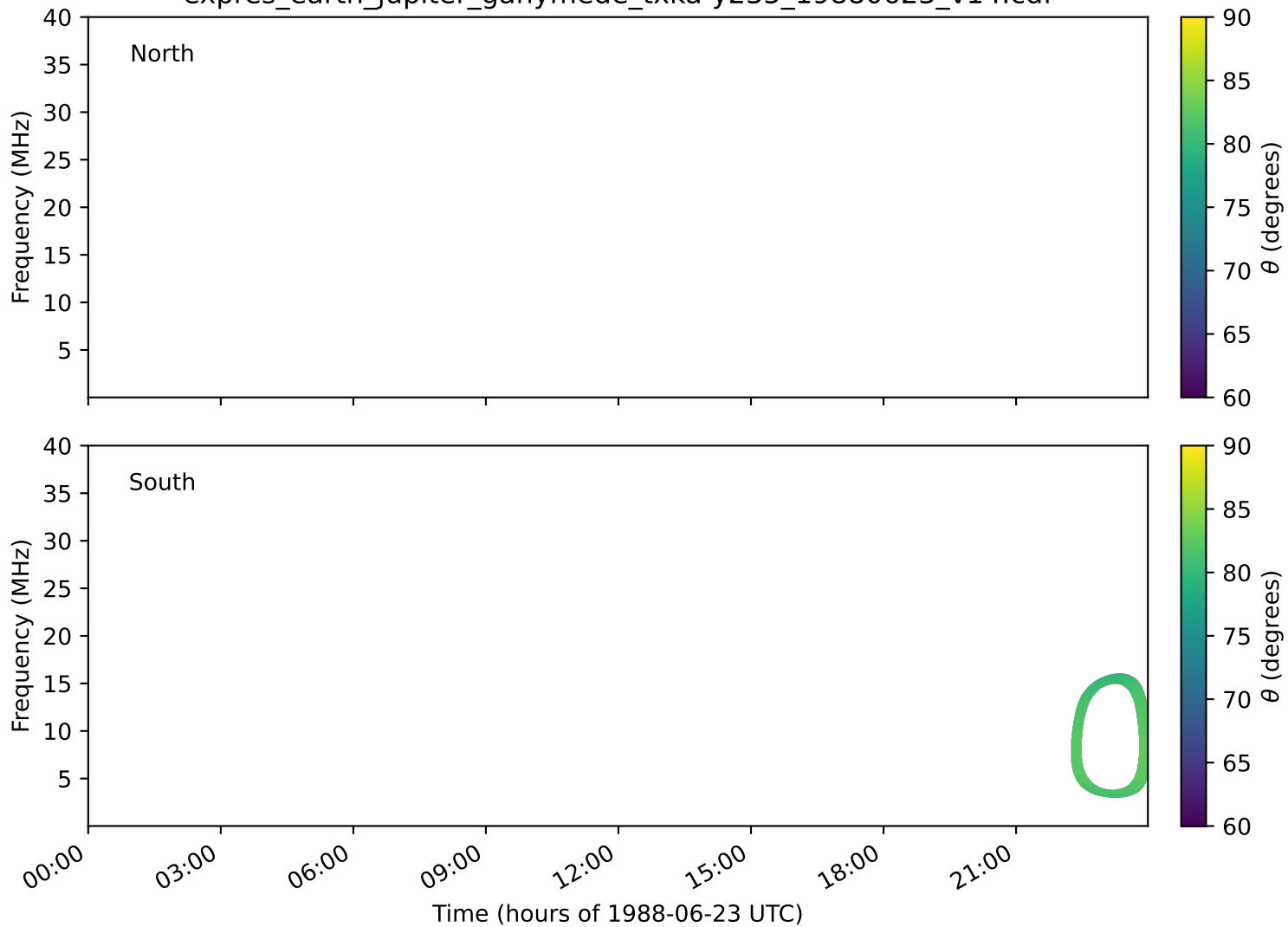
expres_earth_jupiter_ganymede_txka-y235_19880623_v14.cdf
