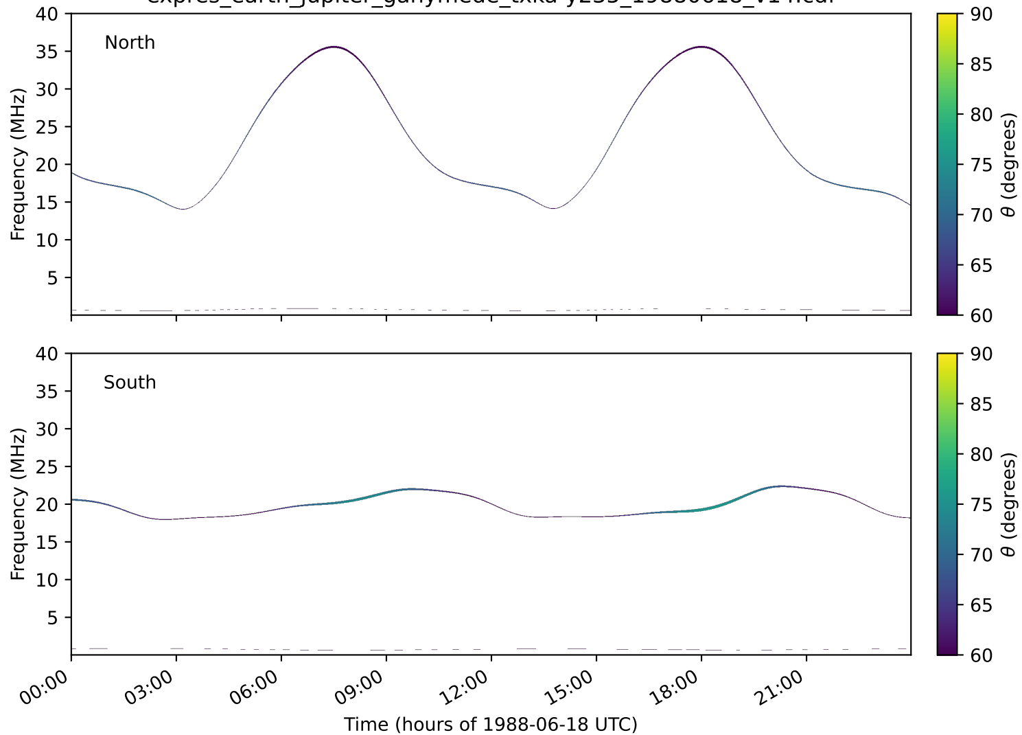
expres_earth_jupiter_ganymede_txka-y235_19880618_v14.cdf
