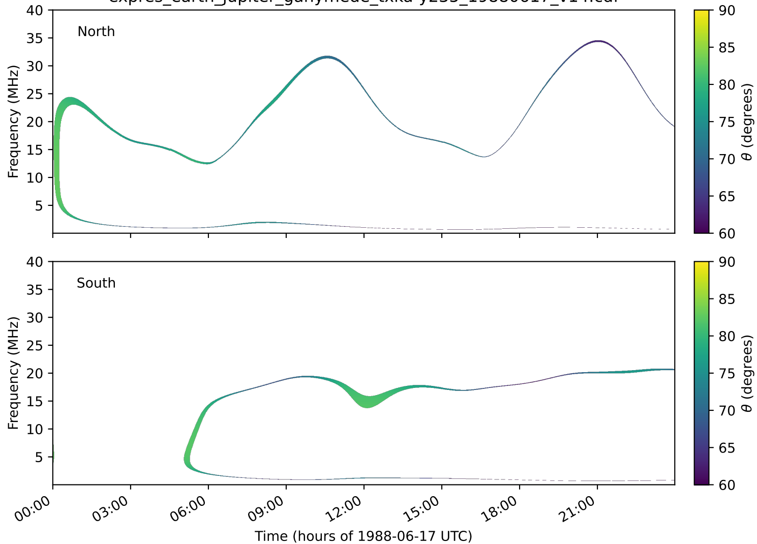
expres_earth_jupiter_ganymede_txka-y235_19880617_v14.cdf
