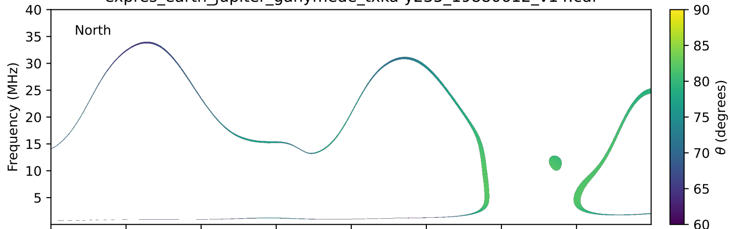
expres_earth_jupiter_ganymede_txka-y235_19880612_v14.cdf
