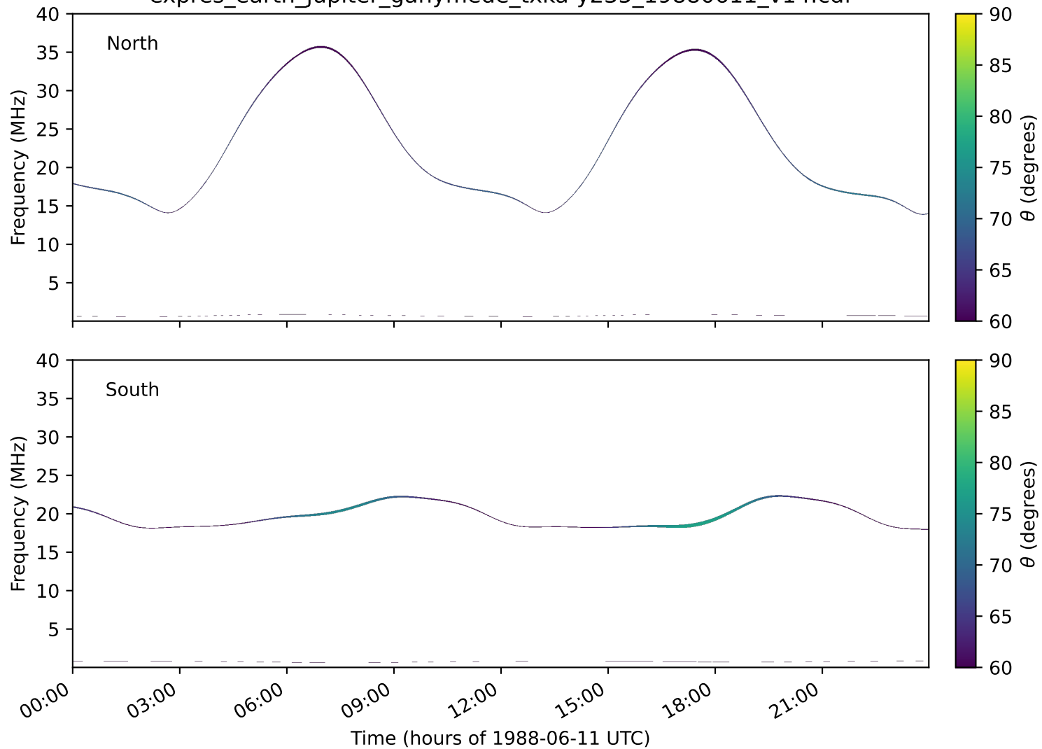
expres_earth_jupiter_ganymede_txka-y235_19880611_v14.cdf
