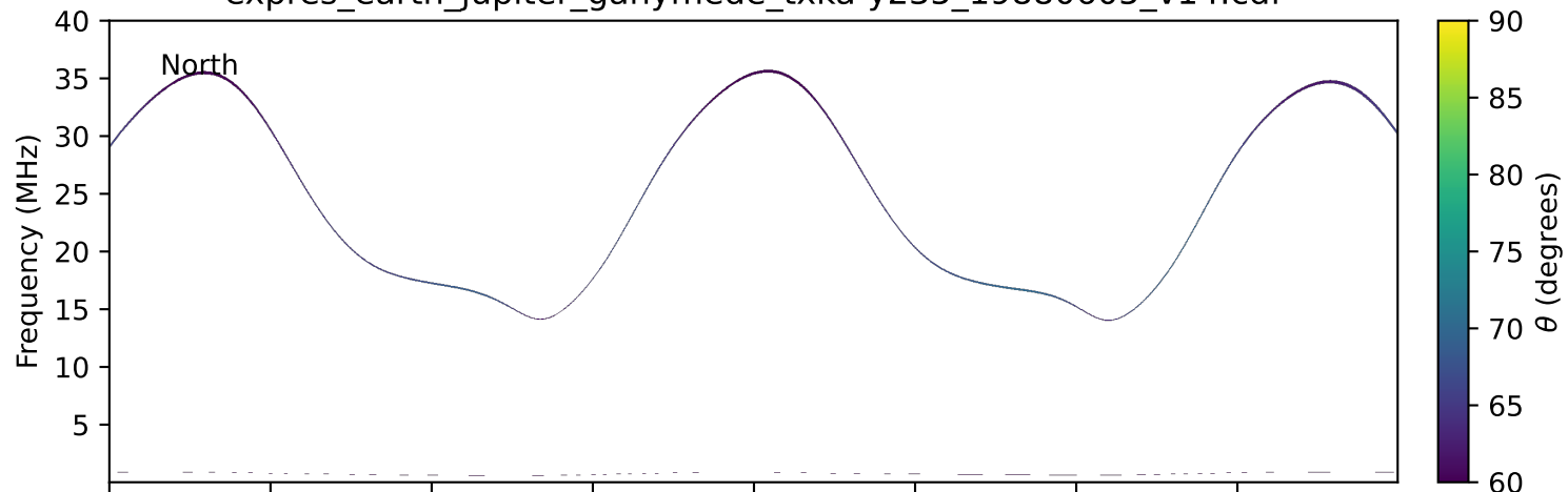
expres_earth_jupiter_ganymede_txka-y235_19880605_v14.cdf
